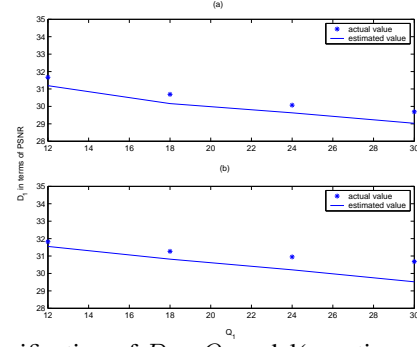
Fig. 3. verification of D - Q model(equations (11, 12, 13 and 14): (a) frame 24; (b) frame 12.
