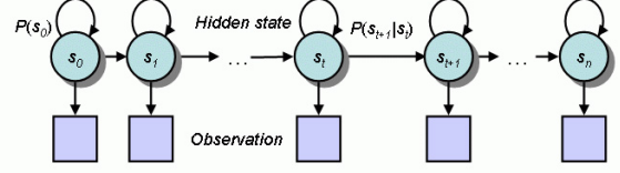
Fig. 4. Left-to-right HMM topology is used for continuous processes.
