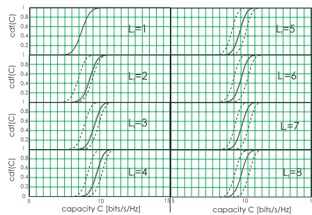
Figure 2. Cdf of the capacity: lower bound (left dashed curves), upper bound (right dashed curves), exact (solid curves), and exact with the use of the simplified selection criterion (solid). N_t = 8 , N_r = 8 , SNR = 20 dB.
