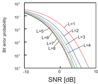
Figure 4. Bit error probability as a function of SNR for Gray-coded \pi/4 -DQPSK as modulation format
