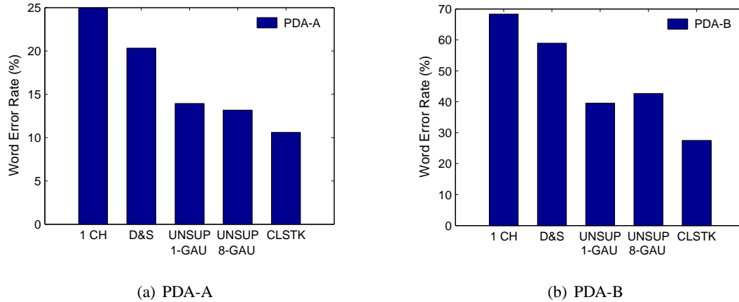
Fig. 5. Word Error Rate obtained using Unsupervised LIMABEAM on the CMU WSJ PDA-A and PDA-B corpora. The figures show the performance obtained using a single microphone, delay-and-sum beamforming, and the proposed Unsupervised LIMABEAM method with 1 Gaussian per state or 8 Gaussians per state in the optimization. The performance obtained using a close-talking microphone is also shown.
