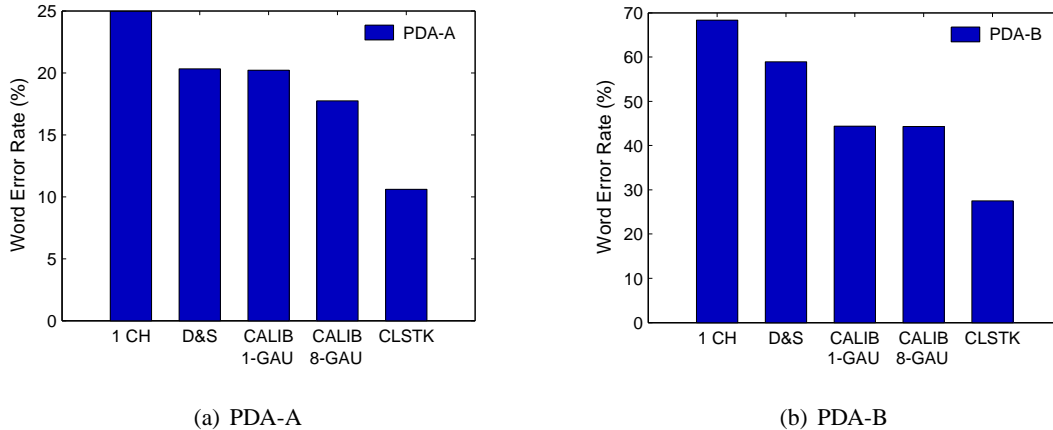
Fig. 4. Word Error Rate obtained using Calibrated LIMABEAM on the CMU WSJ PDA-A and PDA-B corpora. The figures show the performance obtained using a single microphone, delay-and-sum beamforming, and the proposed Calibrated LIMABEAM method with 1 Gaussian per state or 8 Gaussians per state in the optimization. The performance obtained using a close-talking microphone is also shown.
