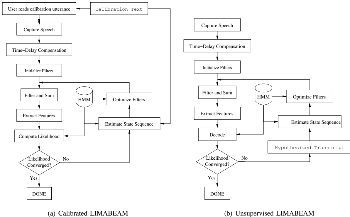
Fig. 2. Flowcharts of Calibrated LIMABEAM and Unsupervised LIMABEAM. In Calibrated LIMABEAM, the parameters of the filter-and-sum beamformer are optimized using a calibration utterance with a known transcription and then fixed for future processing. In Unsupervised LIMABEAM, the parameters are optimized for each utterance independently using hypothesized transcriptions.
