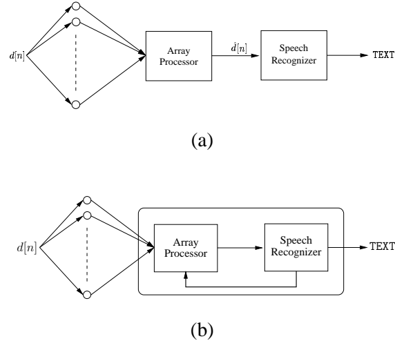
Fig. 1. (a) Conventional architecture used for speech recognition with a microphone array front-end. The objective of the array processor is to estimate the clean waveform . (b) An architecture for array processing optimized for speech recognition. The array processor and the speech recognizer are fully connected, allowing information from the recognizer to be used in the array processing. Note that the system no longer attempts to estimate the clean waveform.
