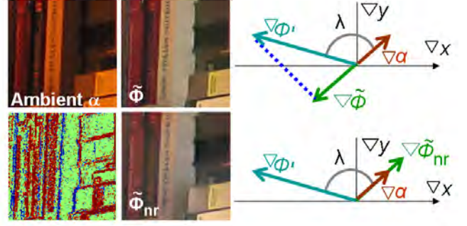
Figure 4: Gradient direction reversal at depth edges. (Left) The top-left patch of the ambient image shown in Figure 2, and the corresponding \cos(\lambda) map (color-coded, red=1, blue=-1). Negative values mostly correspond to depth edges with opposite gradient orientation in flash and ambient images. (Middle) Reconstructed images where the direction of the projected gradient was reversed/not-reversed ( \tilde{\Phi}/\tilde{\Phi}_{nr} ) at depth edges with \lambda > \pi/2 . Notice the jagged depth edges in \tilde{\Phi}_{nr} . (Right) Flash and ambient image gradients for \lambda > \pi/2 . At depth edges, the direction of the projected gradient is reversed to obtain the correct \nabla \tilde{\Phi} (top). If the direction is not reversed (bottom), depth edges are smeared in the reconstructed image.
