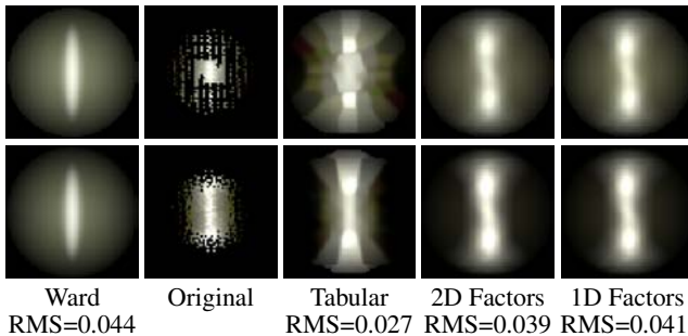
Figure 19: Analysis of the error introduced by several levels of our tree-structured decomposition for BRDFs, and comparison with Ward fits. For each material, the top and bottom rows show parabolic maps of \omega_i distributions at (\theta_d = 15^\circ, \phi_d = 90^\circ) and (\theta_d = 45^\circ, \phi_d = 90^\circ) respectively.
