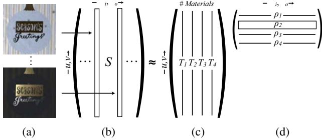
Figure 2: We cast the SVBRDF decomposition depicted in Tree 1 as the factorization of a matrix. (a) High-dynamic range images of a SVBRDF captured with a spherical gantry are (b) organized into a matrix with rows that vary along spatial position and columns that vary along incident and outgoing angles. This matrix is factored into the outer product of (c) functions of spatial position (“blending weights”) and (d) functions of incident and reflected directions (i.e., “basis BRDFs” in tabular form). In this example, we factor the SVBRDF of a holiday greeting card into four terms.
