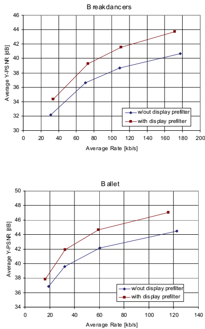
Fig. 4. Comparison of RD curves for breakdancer and ballet sequences when prefiltering is applied with and without display prefiltering.
