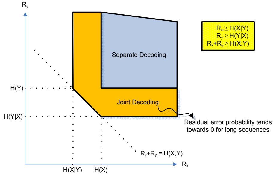
Figure 1: Achievable rates by distributed coding of two statistically dependent random signals.
