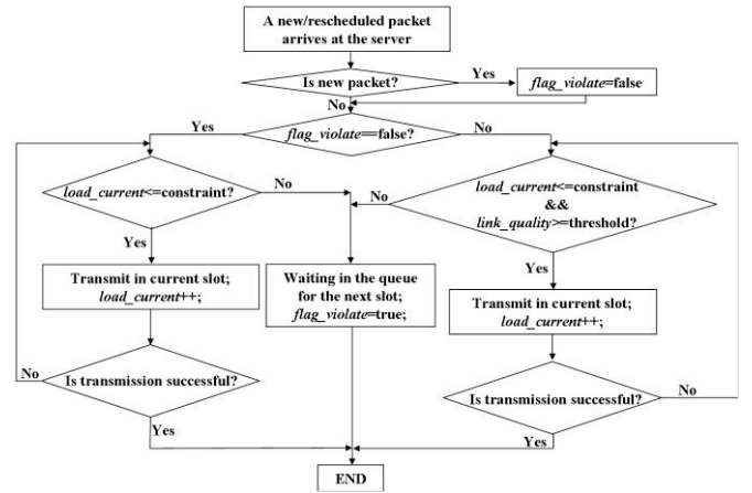
Figure 6. FCFS with peak constraint and partial link reliability.
