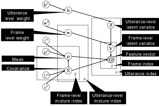
Fig. 3. Graphical representation of multi-scale mixture model.
