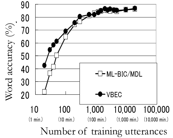
Fig. 1. Superiority of VBEC based acoustic model construction for a small amount of training data.
