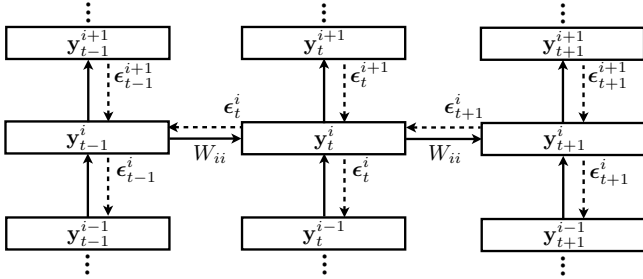
Fig. 2. Backpropagation through time for i^{\text{th}} recurrent layer’s parameter W_{ii} : the solid lines denote the directions of forward propagation and the dotted lines denote the directions of backpropagation.
