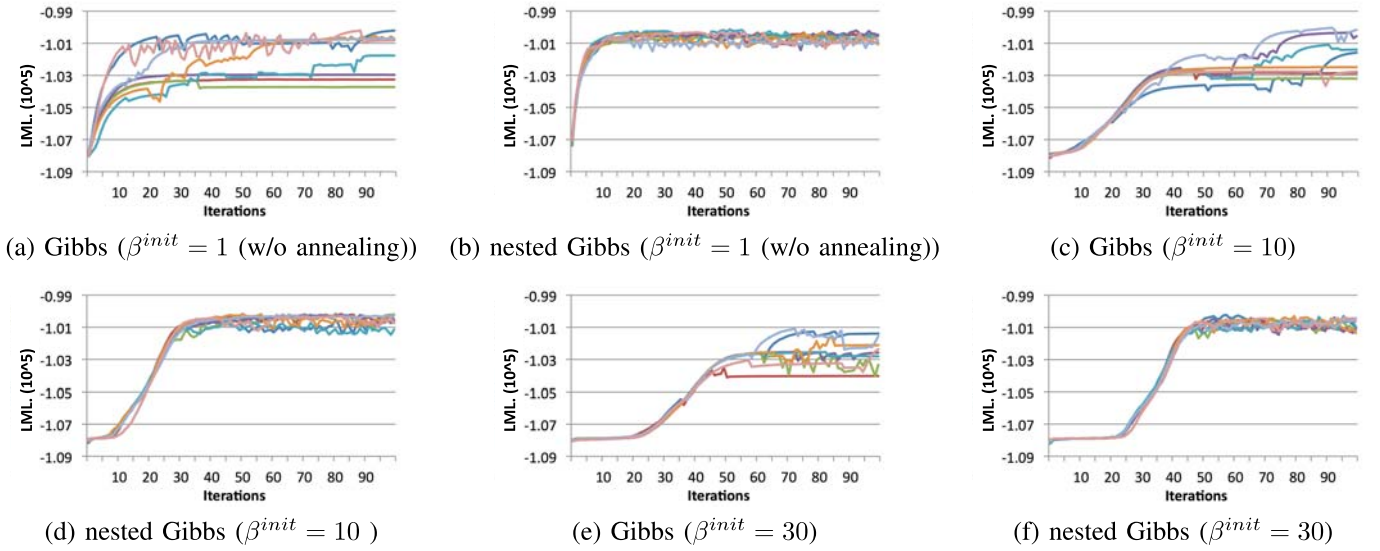
Fig. 6. Logarithmic marginalized likelihood (LML) obtained by Gibbs and nested Gibbs with simulated annealing applied on A1. Each figure shows result with different initial temperature \beta^{init} . Eight lines correspond to the results of eight trials with different seeds.
