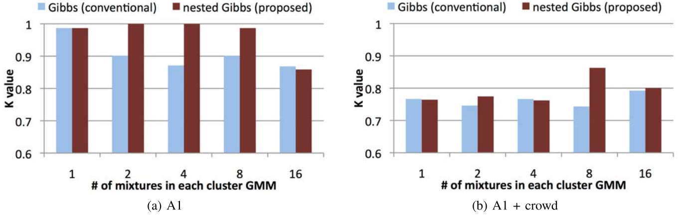
Fig. 5. K values obtained by existing Gibbs and proposed nested Gibbs sampler applied on (a) clean (A1) and (b) noisy (A1 + crowd) speech.
