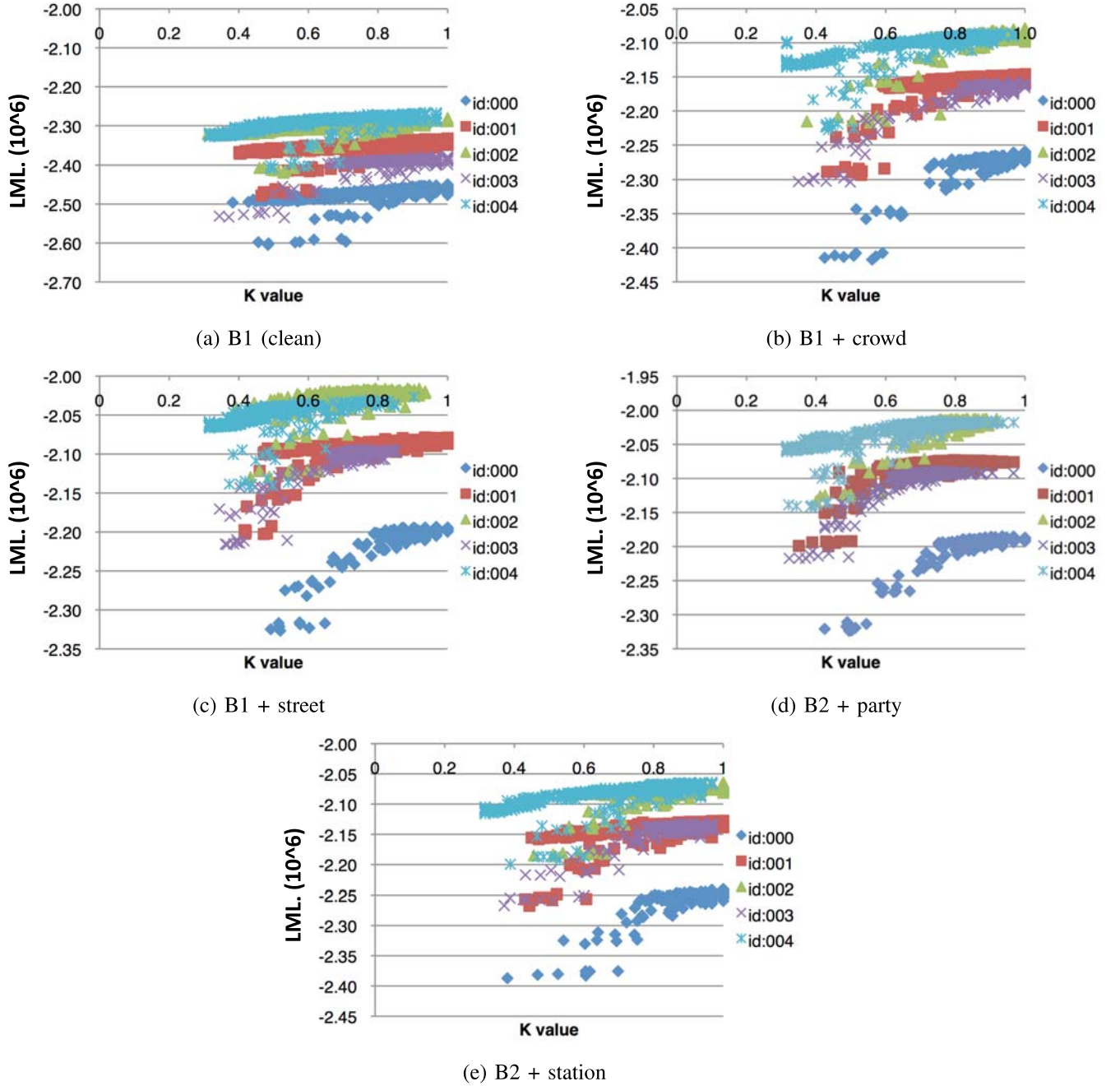
Fig. 4. Logarithmic marginalized likelihood (LML) as a function of K value. Each plot shows the results obtained by applying the proposed n-Gibbs sampler to five different datasets (id:000, 001, ..., 004). Refer to Table I for the details of test set B1.
