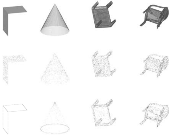
Fig. 4: Haar-like high-pass graph filtering based local variation (2) outperforms pairwise difference based local variation (4). The first row shows the original point clouds; the second and third rows show the resampled versions with respect to two local variations: pairwise difference based local variation (4) and Haar-like high-pass graph filtering based local variation (2), respectively. The two resampled versions have the same number of points—10% of points in the original point cloud.
