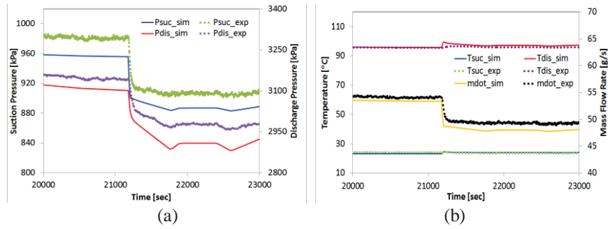
Fig. 3. LEV D opening step response - (a) pressure response; (b) temperature & mass flow rate response
