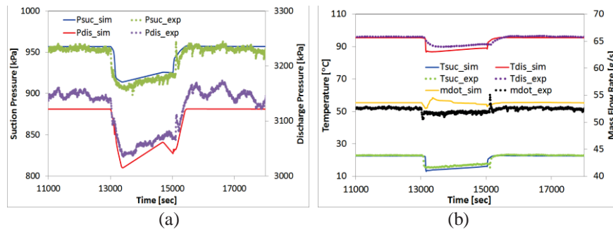
Fig. 5. Indoor fan speed response - (a) pressure response; (b) temperature & mass flow rate response
