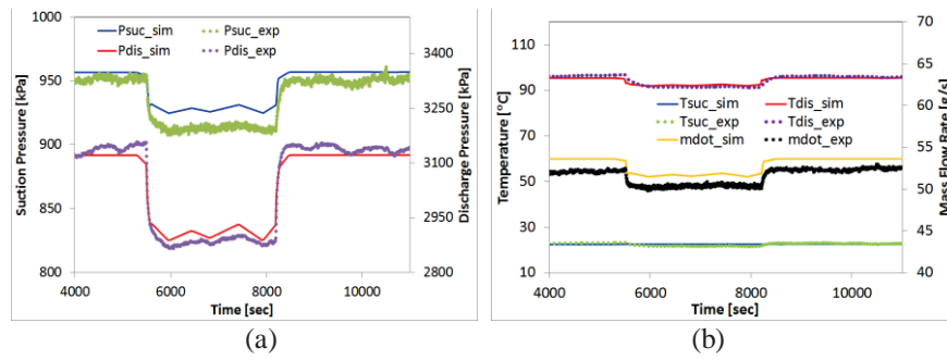
Fig. 4. Outdoor fan speed response - (a) pressure response; (b) temperature & mass flow rate response
