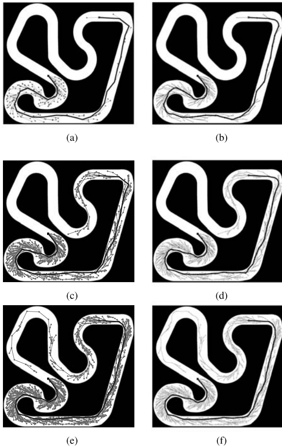
Fig. 2: The evolution of the solution trees for reference paths and state trajectories computed by CL-RRT*, with same notation as in Fig. 1.
