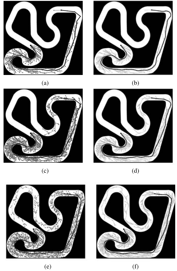
Fig. 1: The evolution of the solution trees for reference paths (a), (c), (e) and state trajectories (b), (d), and (f), computed by CL-RRT # . The trees are at 1000, 2000, and 3000 iterations, respectively.
