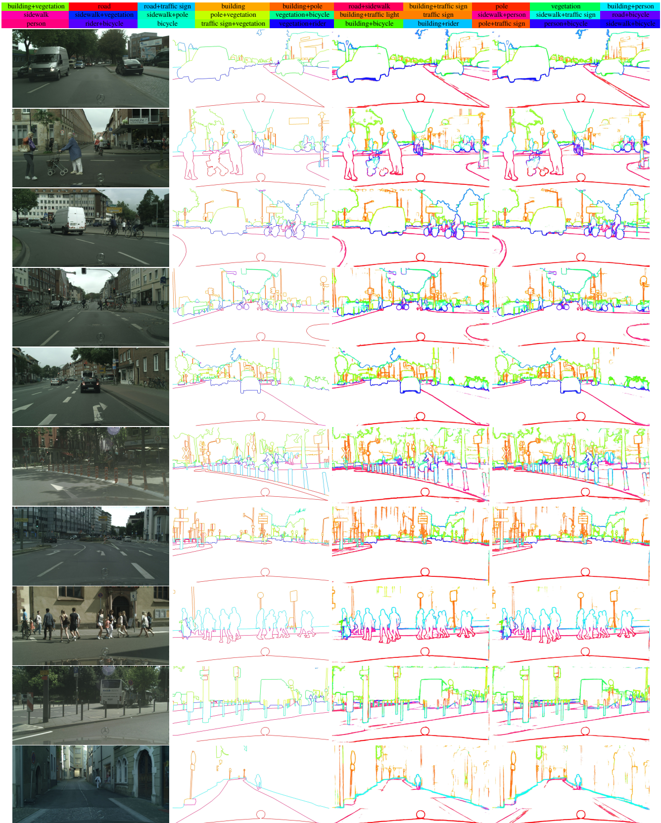
Figure 7. Cityscapes results. From left to right: Input, Ground Truth, result of DSN, and result of CASENet. Visually the result of CASENet and ground truth are very similar. CASENet gets slightly more non-boundary edges and makes minor mistakes near challenging objects like the stroller (2nd row). DSN gets slightly inferior results to CASENet, as observed on more non-boundary edges on the interiors of buildings (e.g., 3rd and 7-th rows). Best viewed in color.
