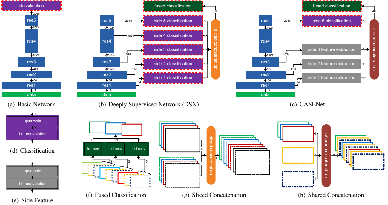
Figure 3. Three CNN architectures designed in this paper are shown in (a)-(c). A solid rectangle represents a composite block of CNN layers. Any change of its width indicates a drop of spatial resolution of this block’s output feature map by a factor of 2. A number besides an arrow indicates the number of channels of the block’s output features. A blue solid rectangle is a stack of ResNet blocks. A purple solid rectangle is our classification module. A dotted red outline indicates that block’s output is supervised by our loss function in equation 1. A gray solid rectangle is our side feature extraction module. A dark green solid rectangle is our fused classification module performing K -grouped 1 \times 1 convolution. (d)-(h) depicts more details of various modules used in (a)-(c), where outlined rectangles illustrate input and output feature maps. Best viewed in color.
