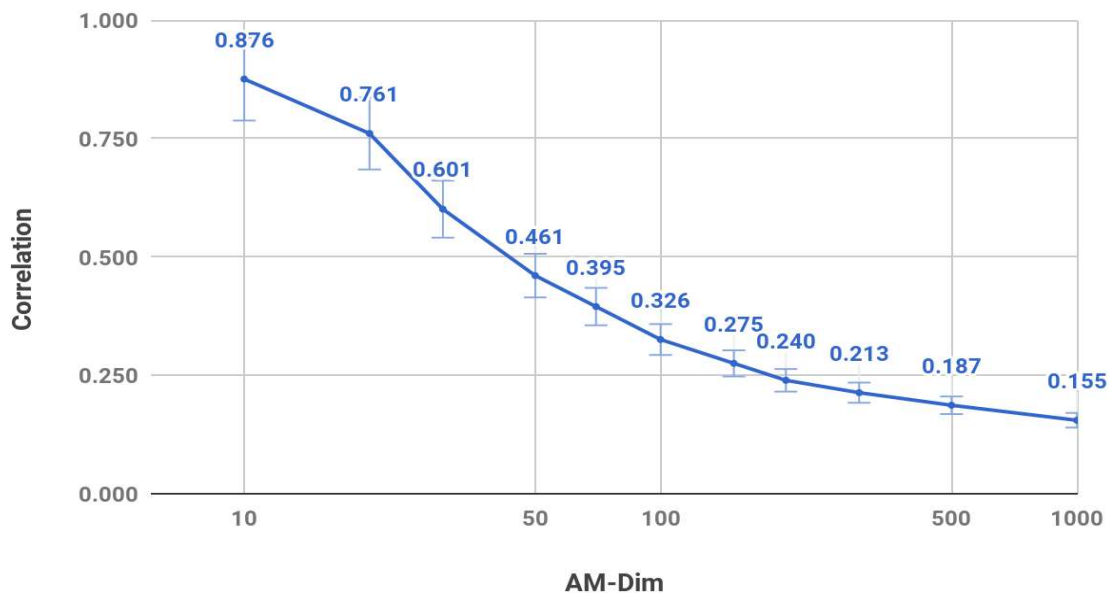
Figure 1. Correlation values for the AM metric as a function of the dimensionality of the embedding
