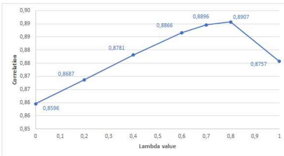
Figure 2. Correlation values for the interpolated AM-FM metric as a function of the interpolation hyper-parameter ( \lambda ). In the figure, a higher value of \lambda gives more weight to the AM component than to the FM component.
