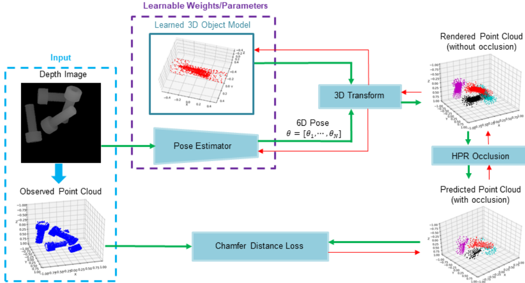
Figure 1. Overview of our unsupervised approach for 3D object model learning and 6D pose estimation. The pose estimator takes as input a depth image, then regresses a 6D pose \theta_i for each object instance i . The learned 3D object model is rendered using the estimated poses. The predicted point cloud is obtained by removing the occluded points from the rendered point cloud using HPR occlusion. The chamfer distance between the predicted and the observed point cloud is used to drive the learning process. We denote forward propagation through the model using green arrows, and backpropagation using red. (Best viewed in color.)
