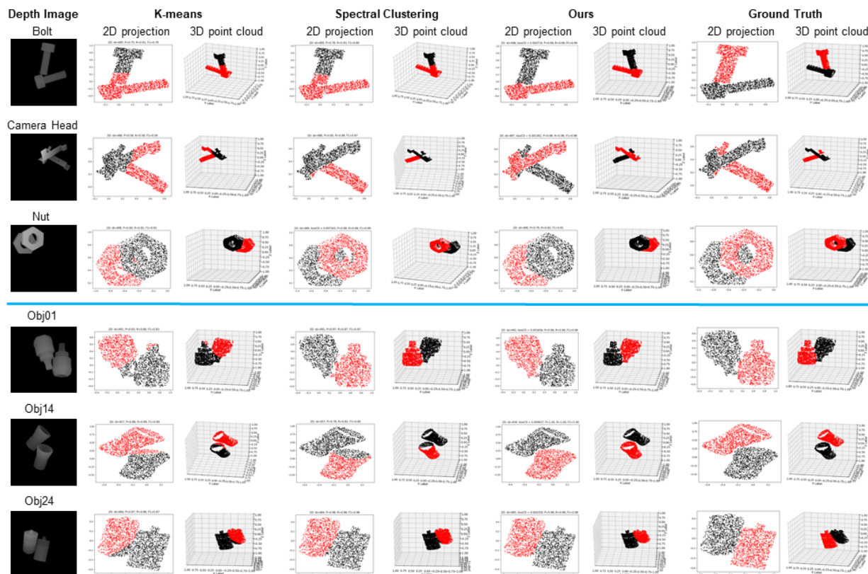
Figure 8. The qualitative results of instance segmentation with N = 2 instances. The object model is learned using one-rotation channel. The 2D projection is obtained by projecting the 3D point cloud into 2D plane.
