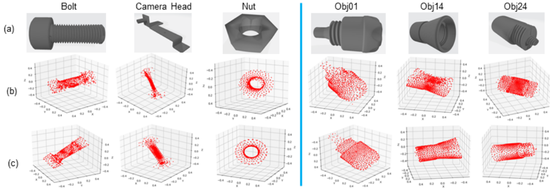
Figure 3. 3D object models that our method learned for six industrial objects from depth images containing one instance ( N = 1 ). (a) True object CAD models, compared with the 3D object models learned using the setting of (b) one rotation channel or (c) two rotation channels.
