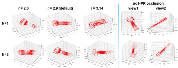
Figure 6. Left : The learned 3D object models using the simplified two-rotation-channel setting, with different values of radius r in HPR occlusion, with N = 1 (top) and N = 2 (bottom) instances of the Bolt. Right : Two views of the 3D object models learned without HPR occlusion for N = 1 (top) and N = 2 (bottom).
