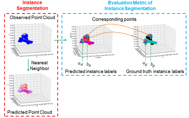
Figure 2. The pipeline of instance segmentation in 3D point clouds, and the evaluation metric of instance segmentation. For every point in the observed point cloud S , we assign to the point the instance label of its nearest neighbor in the predicted point cloud. The performance of instance segmentation is evaluated by calculating the pairwise F1 score.
