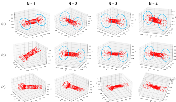
Figure 7. The learned 3D object models of Bolt using the (a) one-rotation-channel, (b) two-rotation-channel, and (c) simplified two-rotation-channel setting, for different numbers of instances N .
