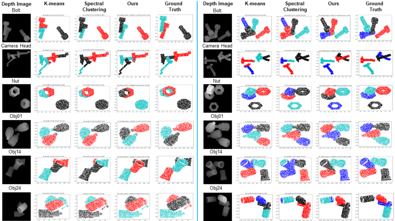
Figure 4. The qualitative results of instance segmentation of 3D point clouds with N = 3 (left) and N = 4 (right) instances.
