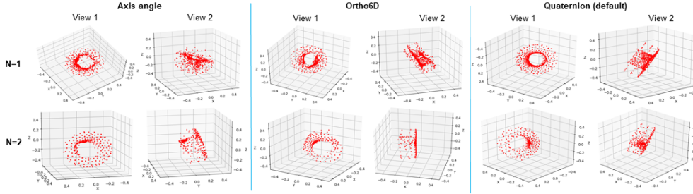
Figure 5. Effect of the algorithm’s rotation representation on the learned 3D object model. The learned 3D object model is shown from two different views for N = 1 (top) and N = 2 (bottom) instances of the Nut.
