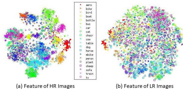
Figure 1. The tSNE [19] of deep features (2048-D) of VOC2007 train set extracted from pool5 layer of pre-trained resnet-101 [12]. (a) Feature of High Resolution (HR) images, and (b) feature of Low Resolution images. The HR features are well separated, however, the LR features are mixed together.
