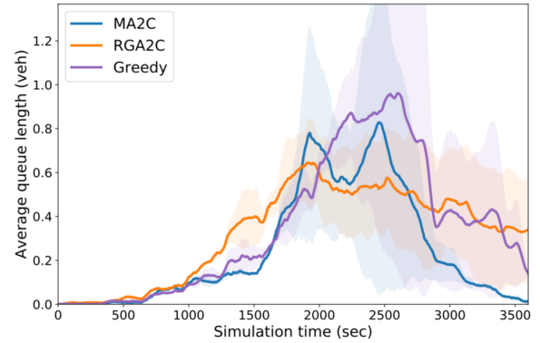
Fig. 8. Average queue length of MA2C (blue), RGA2C (orange), and greedy algorithm (purple) plotted with error bounds (shaded)
