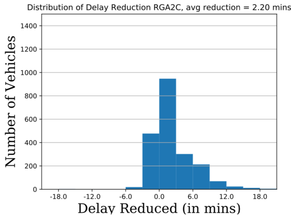
Fig. 9. RGA2C improvement in trip delay compared to greedy algorithm
