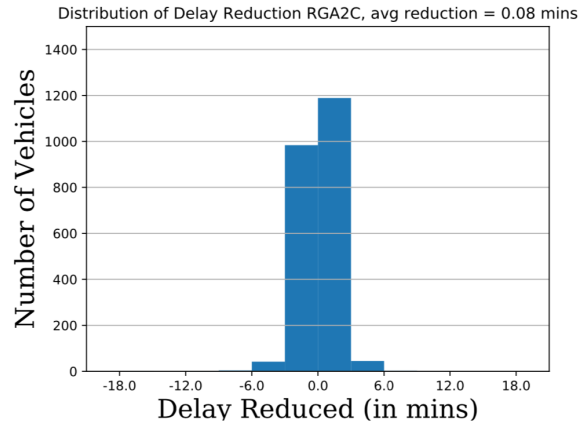
Fig. 10. RGA2C improvement in trip delay compared to MA2C algorithm
