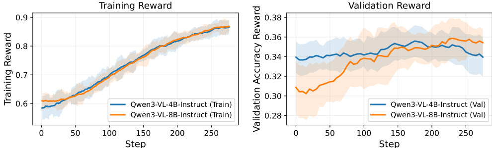
Figure 44: Training and validation reward curves for Qwen3-VL-4B-Instruct and Qwen3-VL-8B-Instruct under GRPO fine-tuning. The 8B model demonstrates greater improvement on the held-out perspective-taking validation task, consistent with its larger capacity. The 4B model shows a slight rise followed by a decline in validation reward, which may indicate partial overfitting to the training domain.
