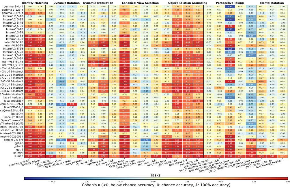
Figure 3: Performance heatmap of 43 VLMs across 26 grouped task variants, organized under 7 spatial reasoning categories. Cohen’s kappa values ( \kappa ) measure chance-adjusted performance, where \kappa = 0 indicates chance-level and \kappa = 1 perfect accuracy. 3 chain-of-thought (CoT) variants of space reasoning models are included for comparison.
