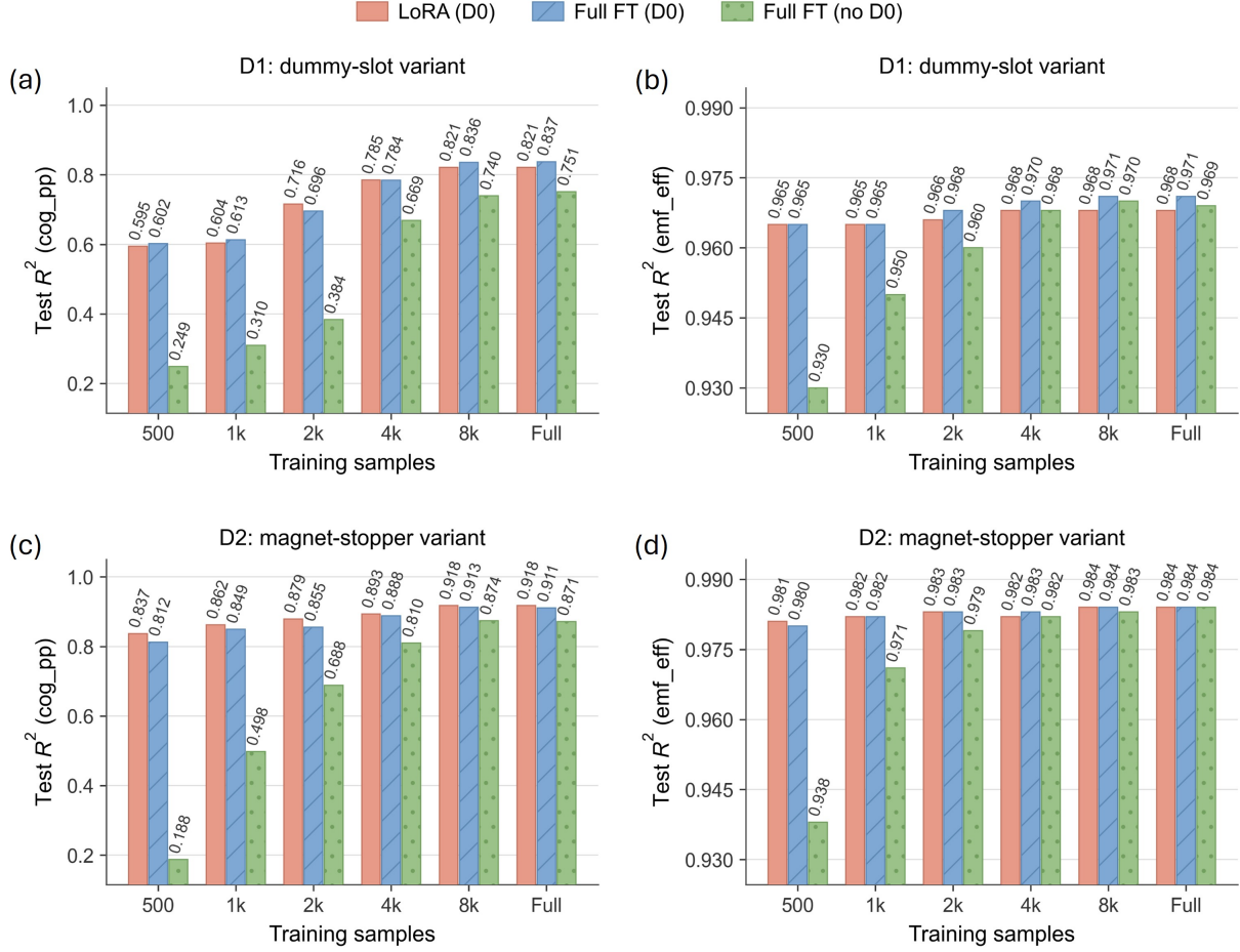
Fig. 4. DistilBERT adaptation under different target-task training sizes on D1 and D2. D0 initialization is most beneficial in the low-data regime, and LoRA remains close to full fine-tuning throughout.
