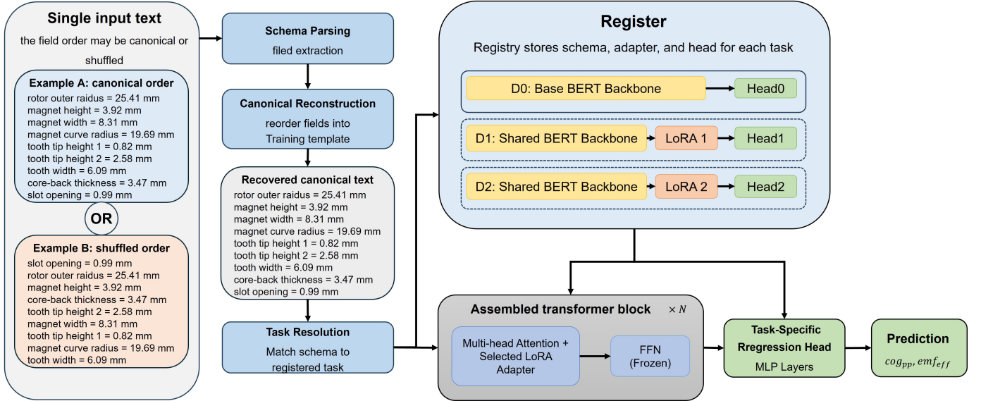
Fig. 3. Schema-guided inference pipeline. The input text may follow either the canonical or a shuffled field order and is first parsed to extract field-value pairs. The extracted fields are then reordered into the canonical training-time sequence. The resulting field set is matched against the registered task schemas, and the registry activates the corresponding LoRA adapter and task-specific regression head on the shared BERT backbone for motor-performance prediction.
