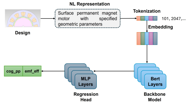
Fig. 2. Text-based surrogate workflow. Motor parameters are serialized into a canonical description, processed by a BERT encoder, and mapped by an MLP head to \text{cog}_{pp} and \text{emf}_{eff} .
