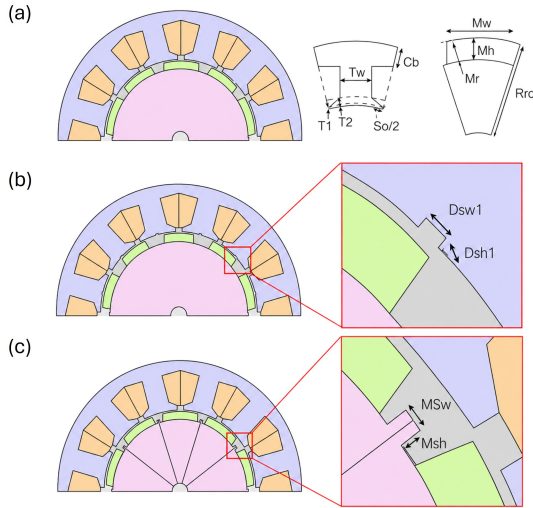
Fig. 1. Three related SPM motor design settings: (a) original design, (b) dummy-slot variant, and (c) magnet-stopper variant.
